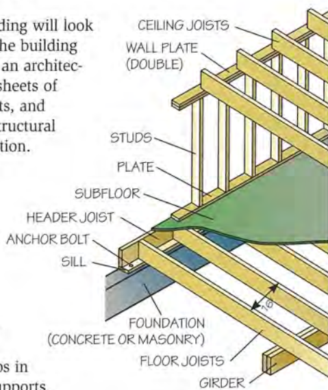
Framing
