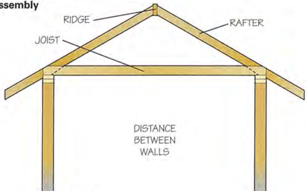
Ceiling joist
