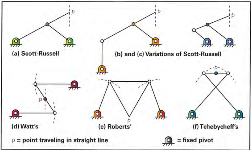
Straight-line mechanisms
