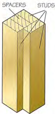
Outside-corner post assembly
